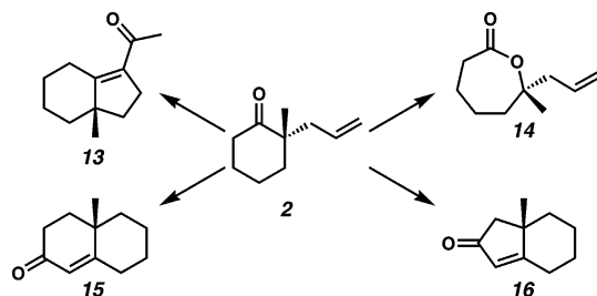
Scheme 1 a
